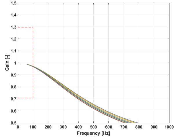
Figure 10 : Frequency response
