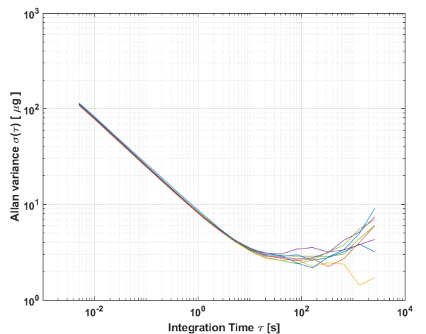
Figure 12: Allan Variance
