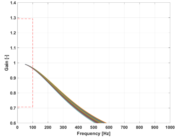
Figure 28 : Frequency response
