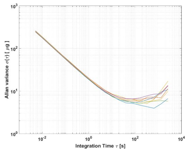
Figure 18: Allan Variance
