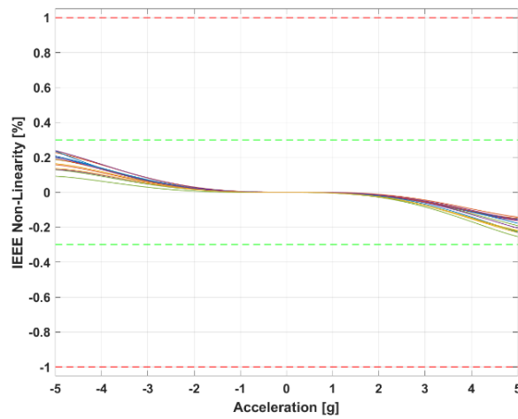
Figure 9 : Non-linearity IEEE
