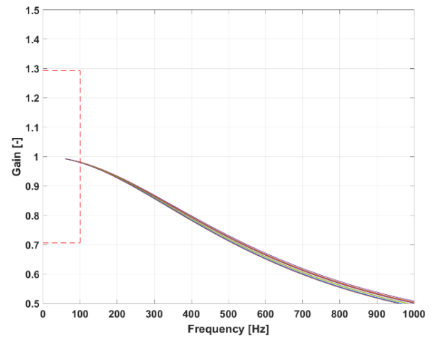
Figure 22 : Frequency response
