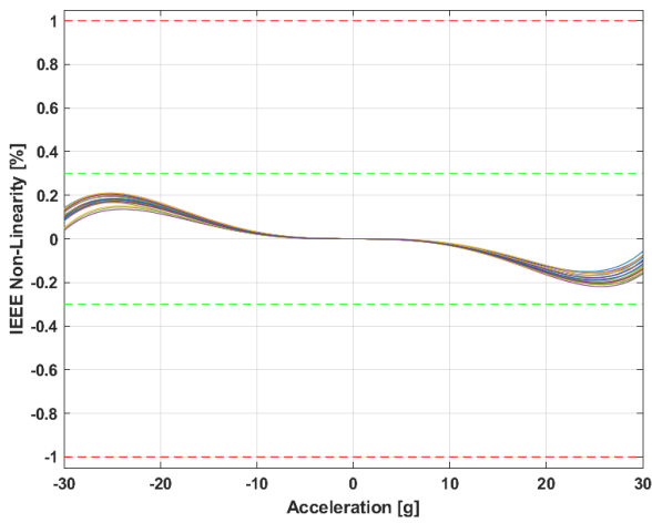
Figure 21 : Non-linearity IEEE
