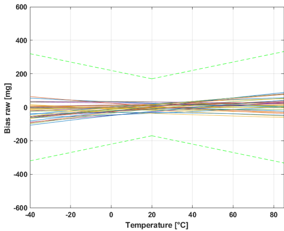
Figure 25: Raw bias
