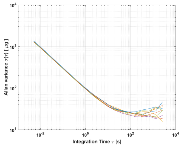
Figure 30: Allan Variance
