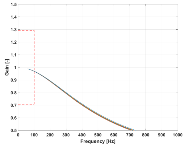
Figure 34 : Frequency response
