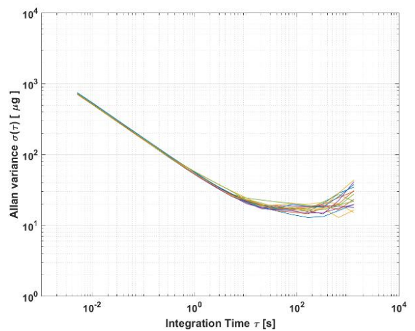
Figure 24: Allan Variance
