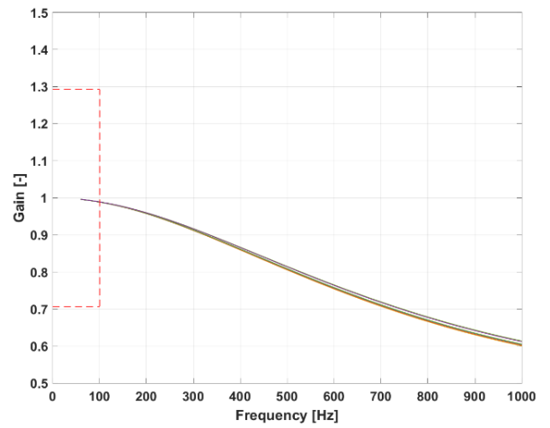
Figure 16 : Frequency response
