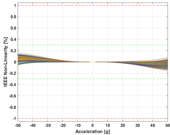
Figure 27 : Non-linearity IEEE
