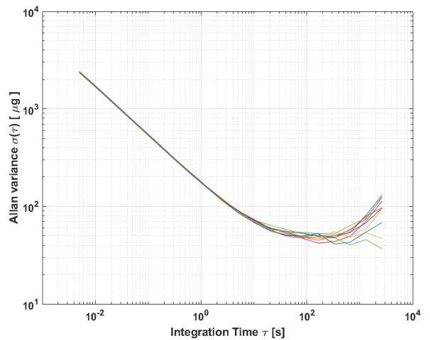
Figure 36: Allan Variance
