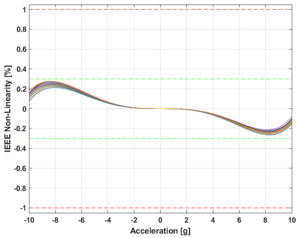
Figure 15 : Non-linearity IEEE
