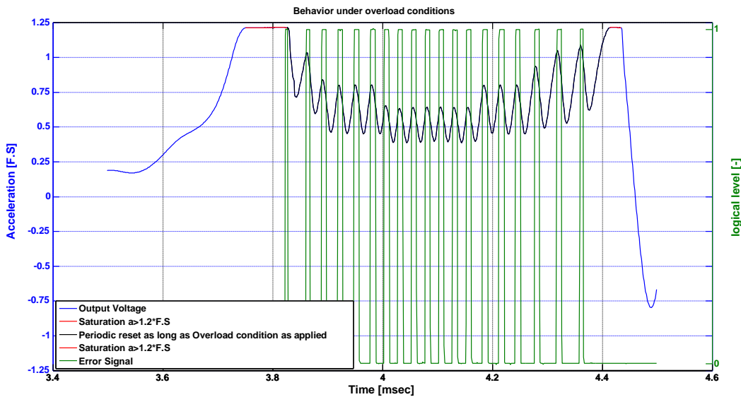
Figure 42 : Overload Behavior
